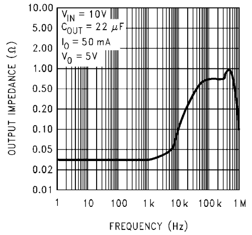
Output Impedance
