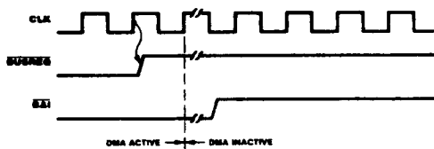
Figure 16. Bus Release (Byte-at-a-Time Mode)
