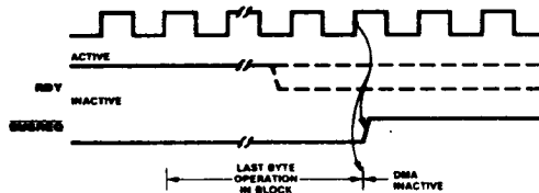
Figure 17. Bus Release at End of Block (Burst and Continuous Modes)
