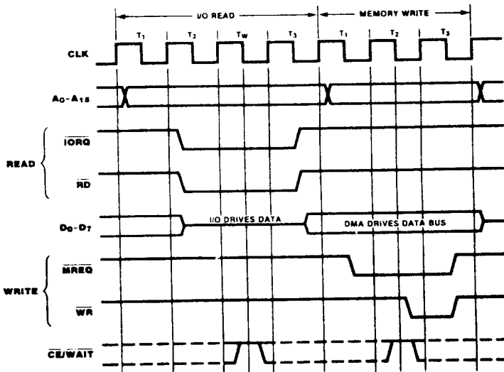
Figure 13. I/O-to-Memory Transfer
