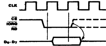
Figure 11. CPU-to-DMA Read Cycle
