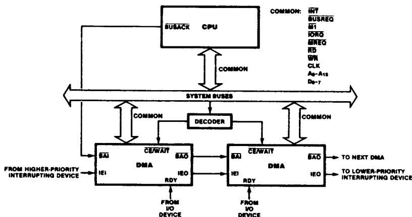
Figure 7. Multiple-DMA Interconnection to the Z-80 CPU
