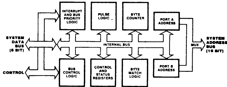
Figure 6. Block Diagram
