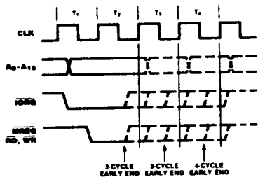
Figure 14. Variable-Cycle and Edge Timing
