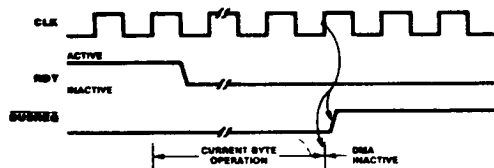
Figure 18. Bus Release When Not Ready (Burst Mode)
