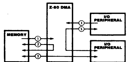
1. Search memory 2. Transfer memory-to-memory (optional search) 3. Transfer memory-to-I/O (optional search) 4. Search I/O 5. Transfer I/O-to-I/O (optional search)
