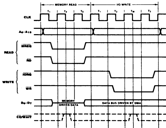
Figure 12. Memory-to-I/O Transfer
