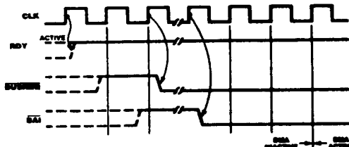
Figure 15. Bus Request and Acceptance
