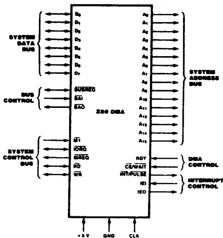
Figure 1. Pin Functions
