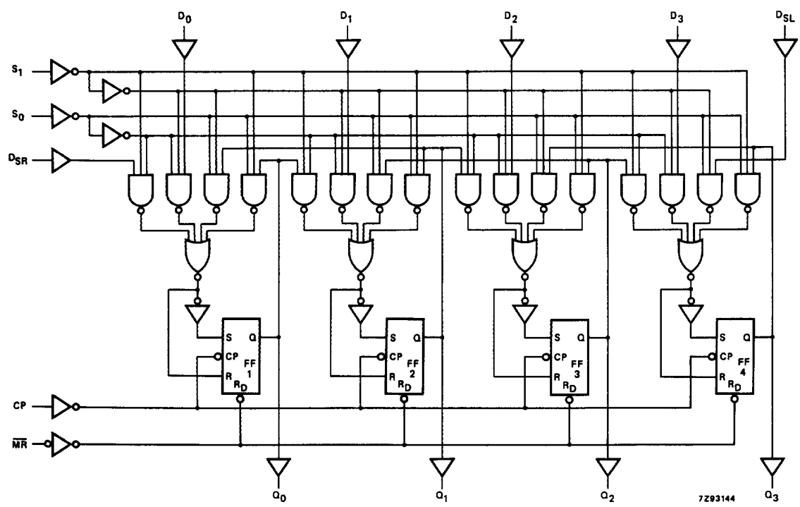
Fig.5 Logic diagram.
