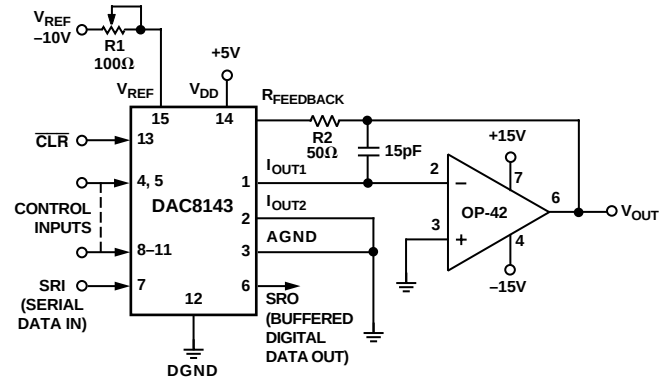
Figure 17. Unipolar Operation with Fast Op Amp and Gain Error Trimming (2-Quadrant)
